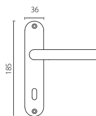
Key (BS)
