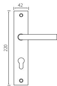
Cylinder (CYL)
